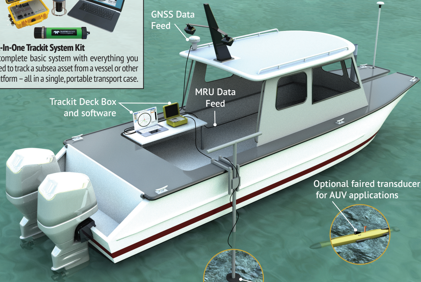
DAT with optional mounting sleeve deployed on customer supplied pole mount
